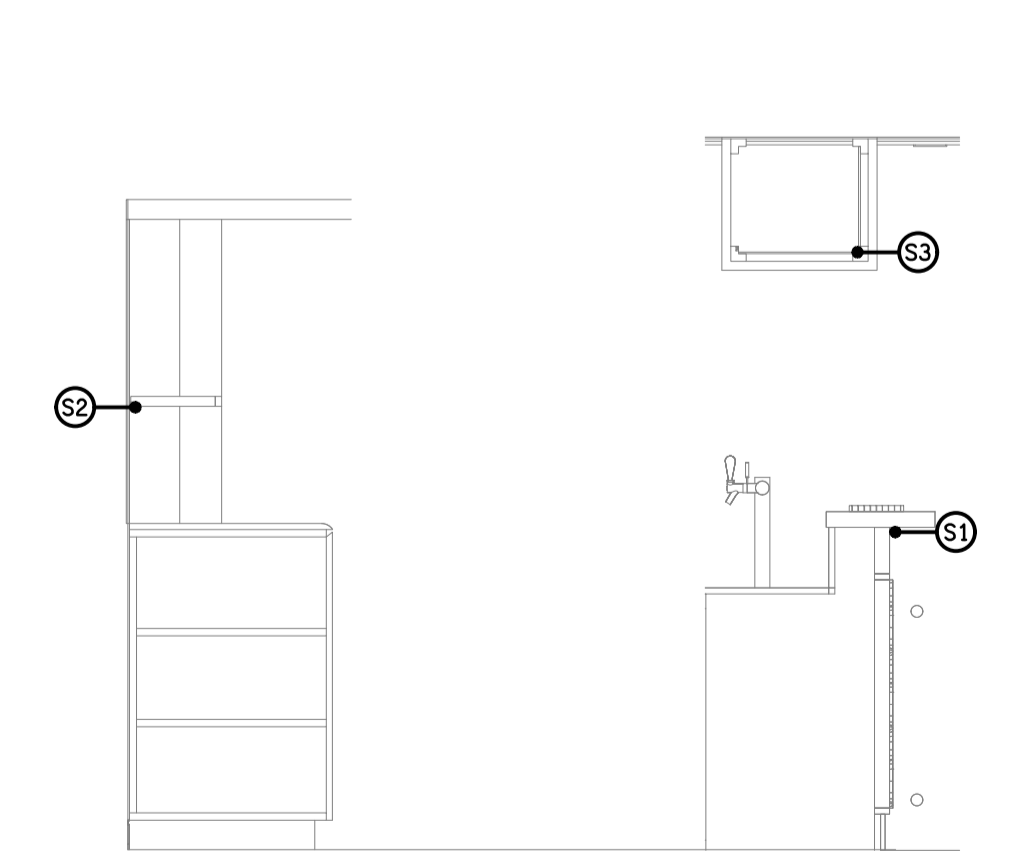
DETAIL B BISTRO BAR SECTION SCALE 1:25
